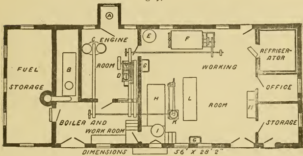
Floor plan of creamery for whole milk.
